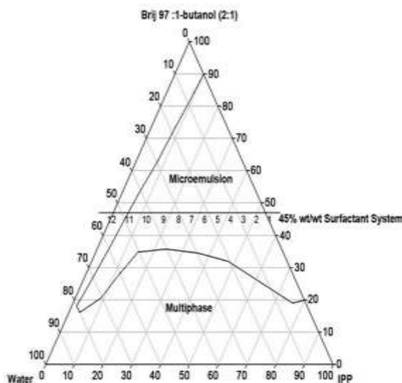
Figure 3 The Pseudoternary Phase Diagram of Ipp/Water/Brij 97:1-Butanol (2:1) And The Dilution Line for Investigation at 45% Wt/Wt Surfactant System 49
