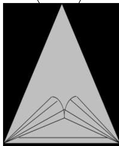
Figure 2 Formulating Microemulsion
